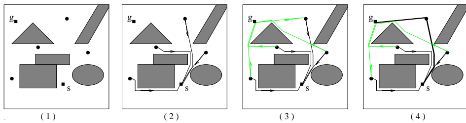
Fig. 2.: An illustrative diagram: (1) Randomly generated subgoals in C-free space; (2) Each process conducts search for a subpath from the subgoal to the start configuration; (3) After step 2, each process starts searching for another subpath from the subgoal to the goal configuration; (4) The first path a process returns will be accepted as the final path.
