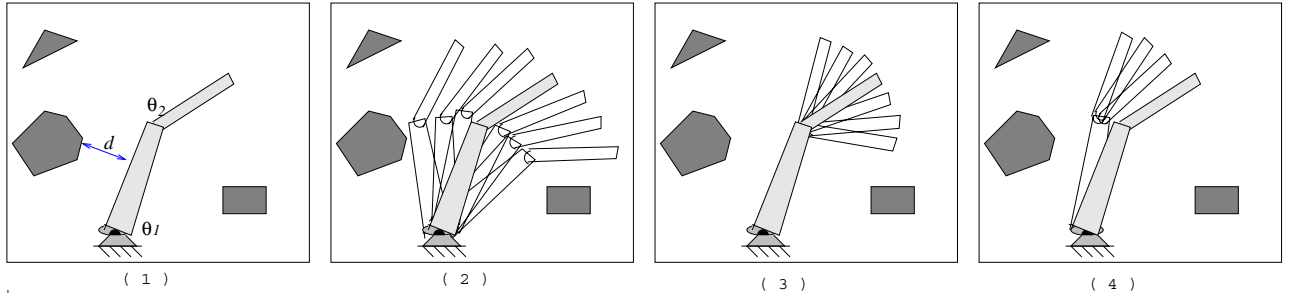
Fig. 3.: An illustration of using the heuristic of prediction of maximum movement with FreeSteps = 3 . (1) The arm's current configuration. (2) The arm is ensured to be collision-free while moving along \theta_1 for 3 consecutive steps in either the positive or negative direction (with \theta_2 fixed). (3) Similar as the above with \theta_1 and \theta_2 exchanged. (4) The arm is collision-free while moving along the coordinate axis (either \theta_1 or \theta_2 ) directions of the C-space for 3 consecutive steps.
