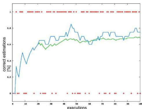
Figure 9: Overall (green) and averaged (blue) percentage of correct estimations of the rod's rotation on the conveyor belt using the change function for 100 executions. A red dot with a value of 0 indicates that the first correction of the rotation did not align the rod perfectly and further corrections were necessary. A red dot with a value of 1 indicates that the rod was aligned correctly with only one motion.
